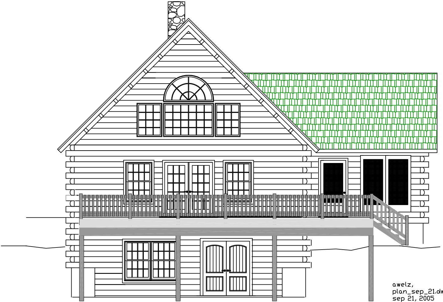
EAST ELEVATION
