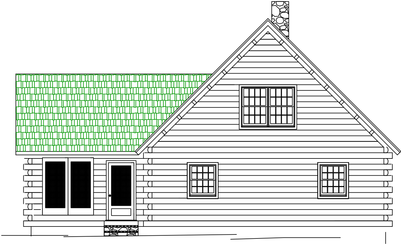
WEST ELEVATION
