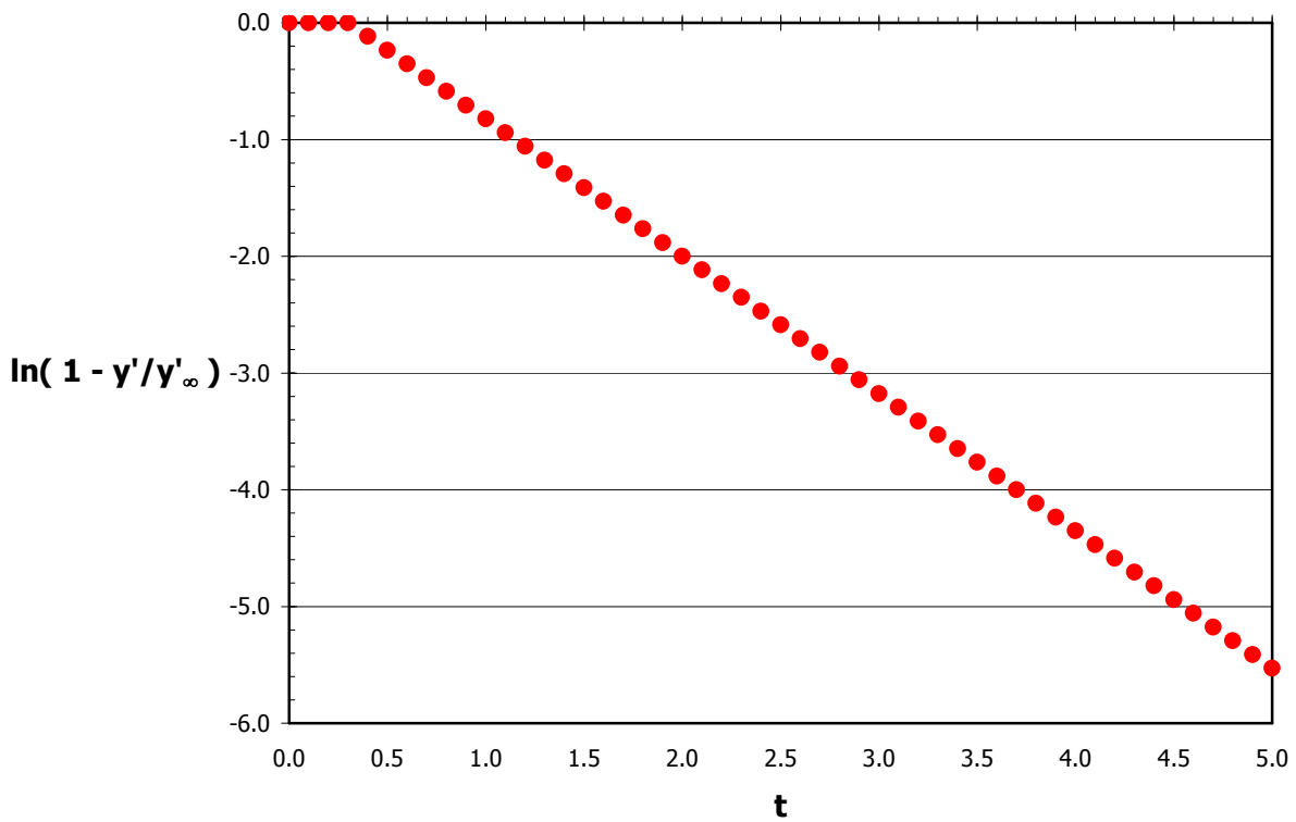
Figure 2. Data Points After Transforming FOPDT Response Equation
