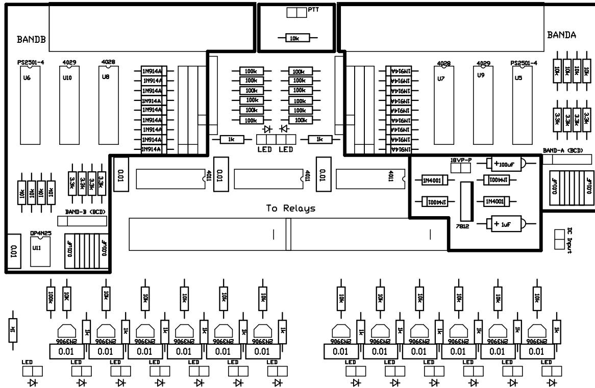
C:\Program Files\CircuitMaker 2000\Circuits\Switch2x6_ControlBoardV4d8wired.PCB Top Overlay
