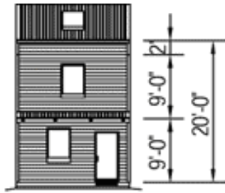
NORTH END ELEVATION
