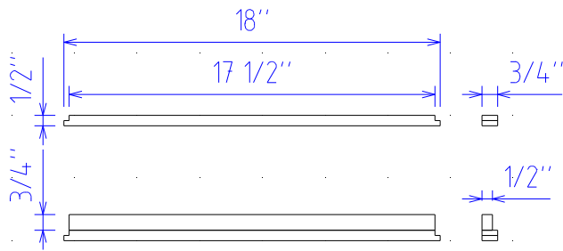
Drawer Guides
