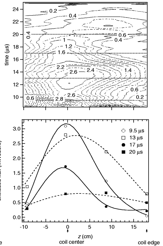
FIG. 8. Excluded flux contours as a function of time and axial position, FRX-L shot 1525 (top), and excluded flux vs axial position at various times (bottom). Lineouts at 9.5 and 13 \mu s correspond to the first peak in the main reversal field and the first minimum of the modulation, respectively (see Fig. 7). Data points (markers) are splined along z .
