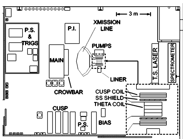
FIG. 2. Layout of FRX-L components, including main, bias, preionization (PI), and cusp capacitor banks, transmission (xmission) line, power supplies (PS), triggers (trigs), stainless steel (SS) shields, theta coils, cusp coils, and liner. (Inset is a closeup of the device central core.)
