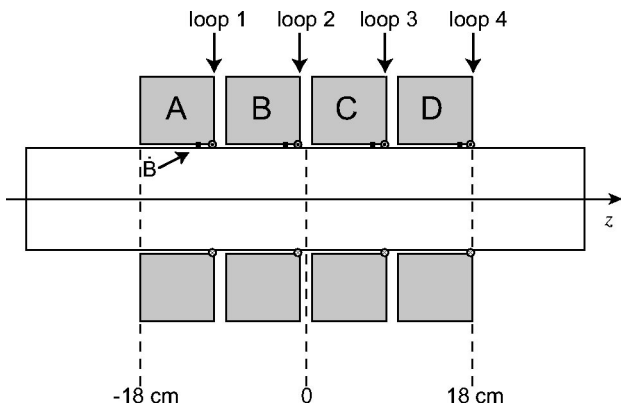
FIG. 6. Cross section of a theta coil showing location of flux loop and \dot{B} probes.
