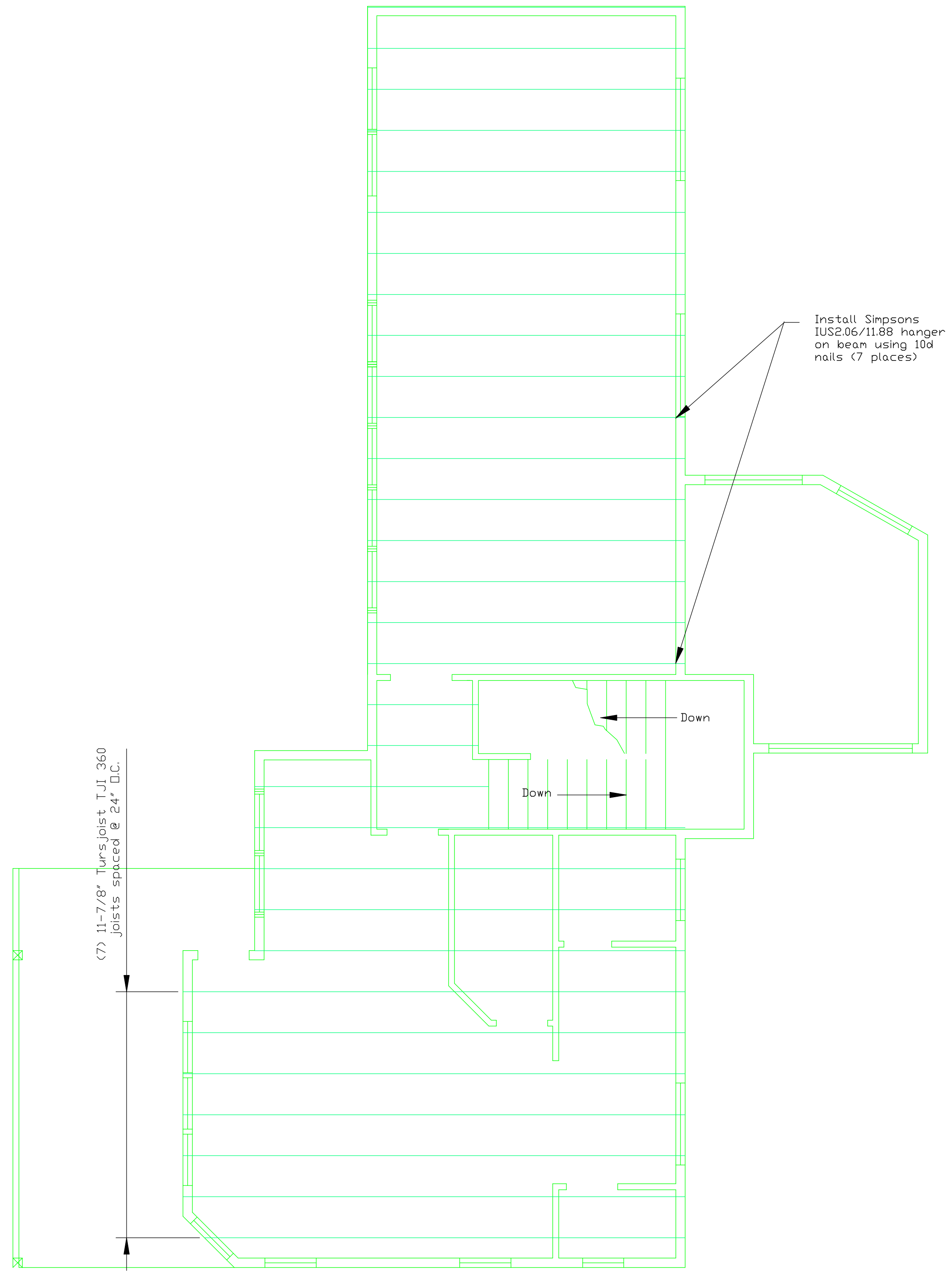
Second floor framing
