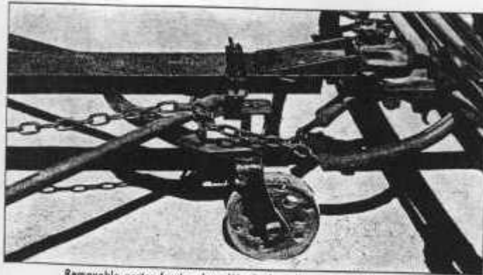
Removable caster for tow bar. (Used when disconnected from car.)
